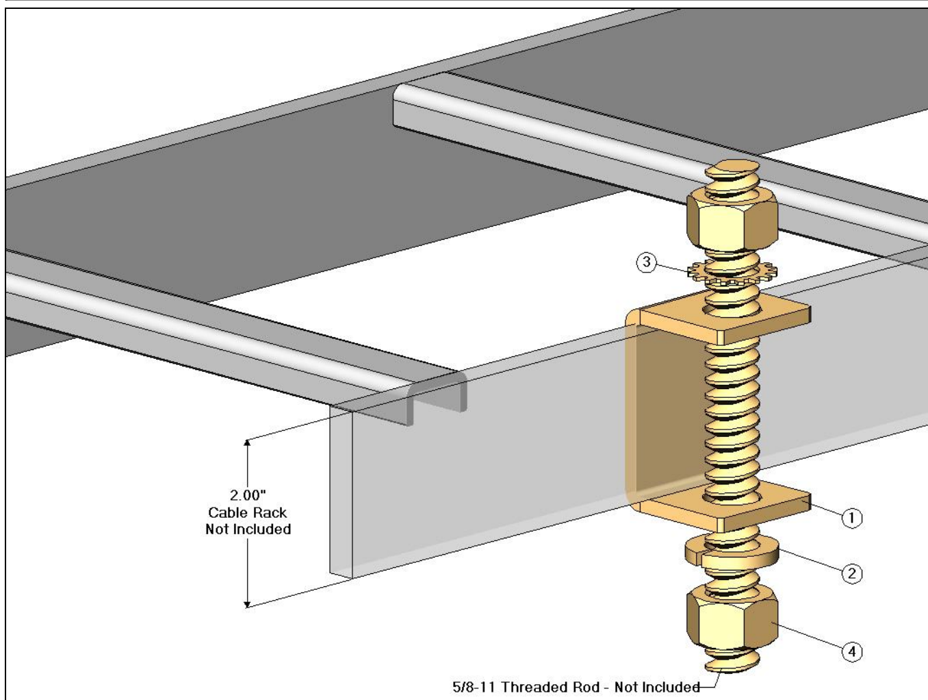
HB2x Series - 2.00" Cable Rack Hanger Kit Selection
